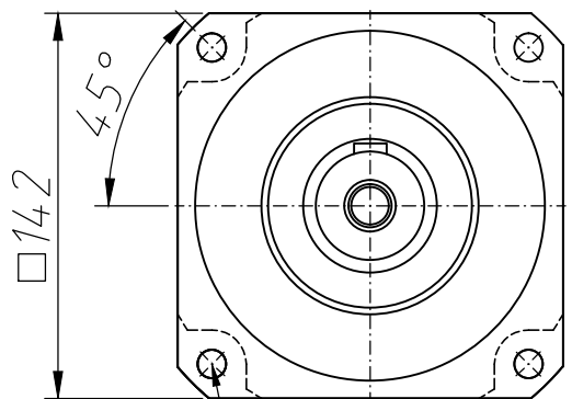
Output shaft
